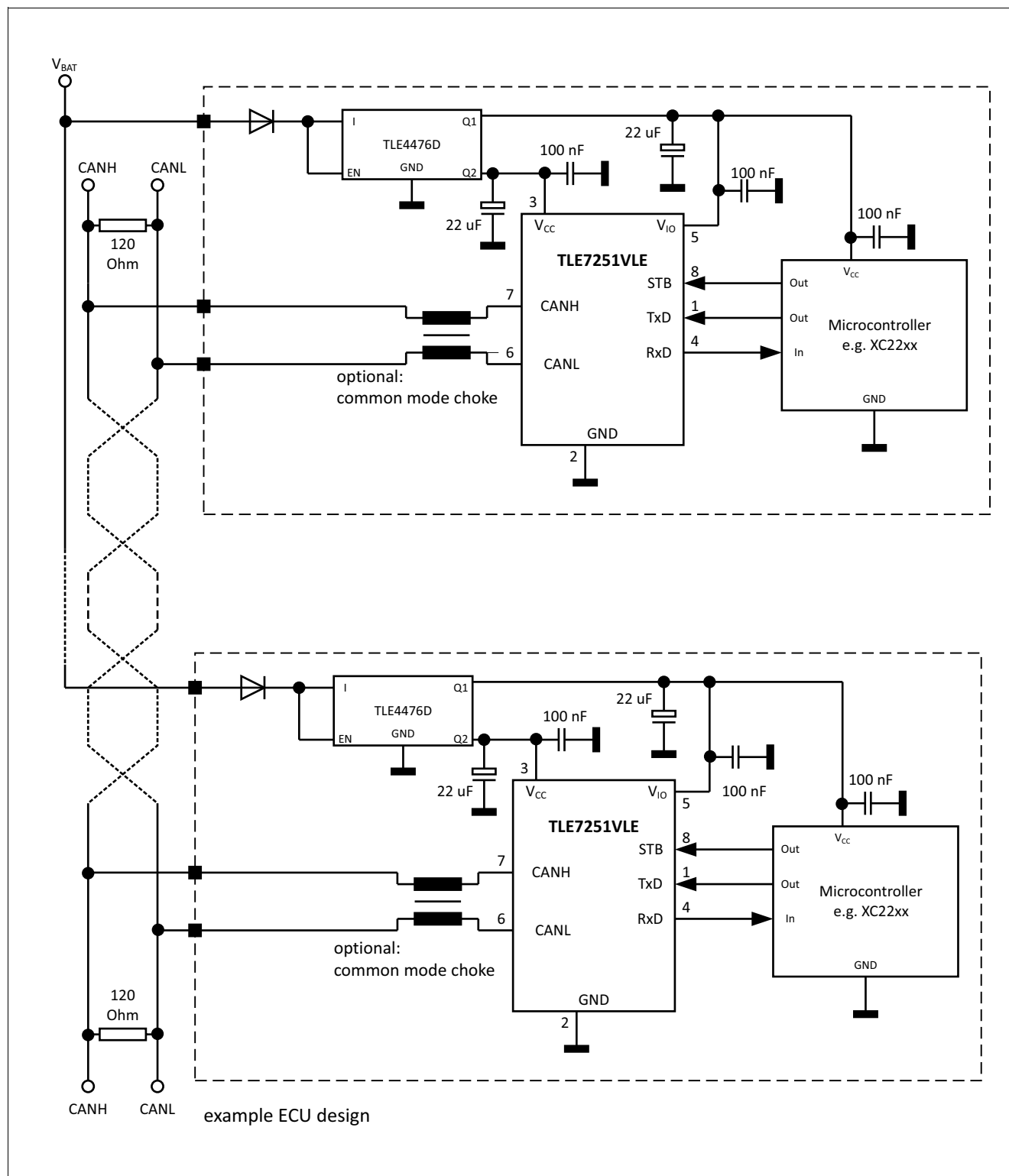
Figure 14 Application circuit
