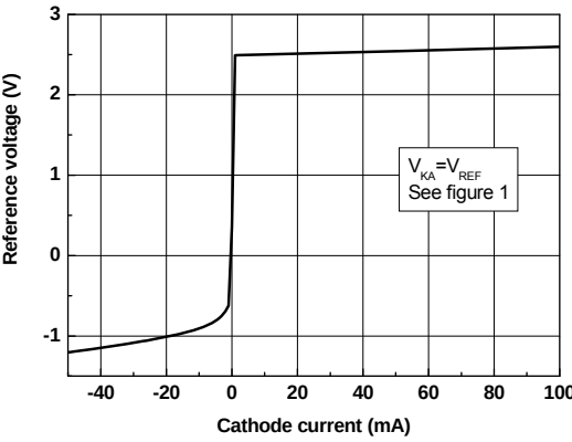
Figure 12. Reference voltage vs. cathode current
