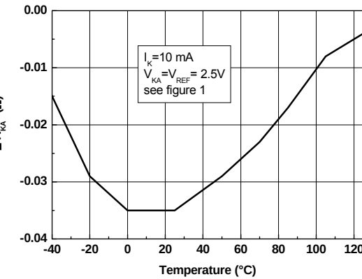
Figure 17. Drift of R_{KA} vs. temperature
