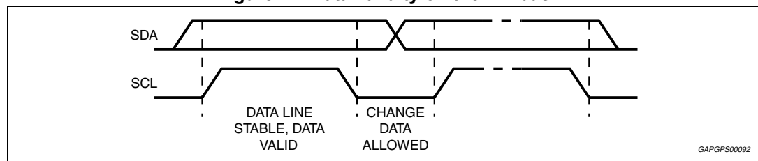
Figure 21. Data validity on the I 2 C bus
