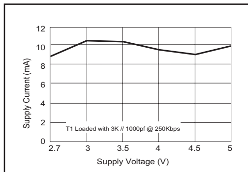
Figure 4. Supply Current vs Supply Voltage for the SP3220EB.
