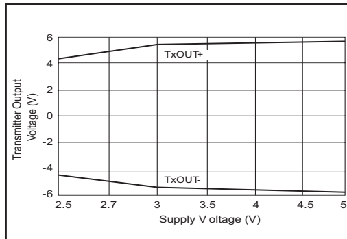
Figure 8. Transmitter Output Voltage vs Supply Voltage for the SP3220EU.
