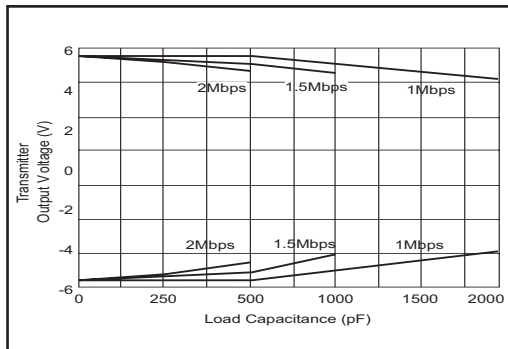
Figure 7. Transmitter Output Voltage vs Load Capacitance for the SP3220EU.
