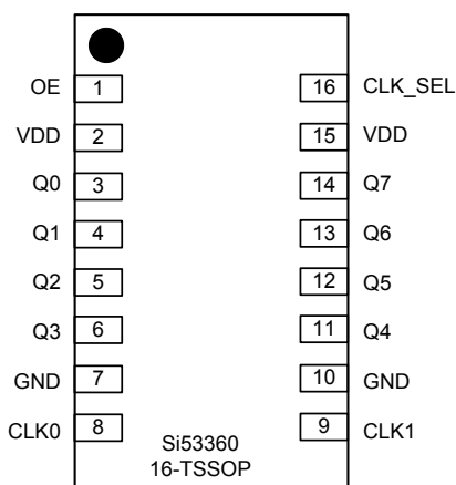
Figure 5.1. Si53360 Pin Descriptions
