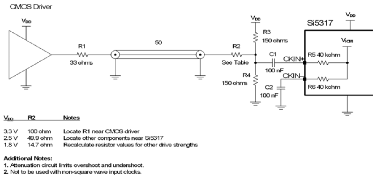
Figure 10. CMOS Termination with Attenuation and AC-Coupling (1.8, 2.5, 3.3 V)
