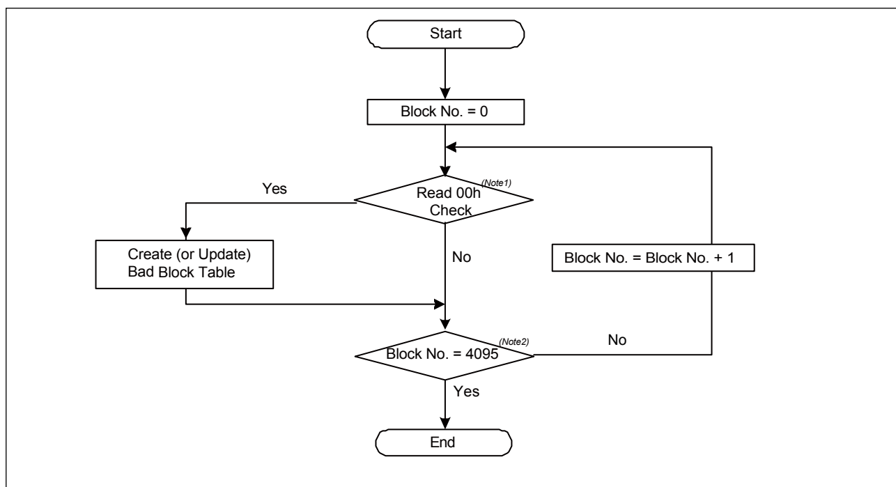
Figure 48. Bad Block Test Flow
