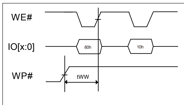
Figure 46-1. Enable Programming of WP# Signal
