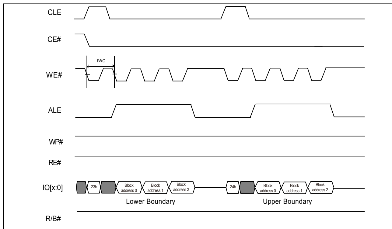
Figure 38. AC Waveforms for Block Unprotection
