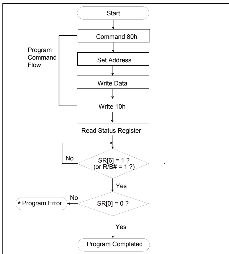
Figure 50. Program Flow Chart
