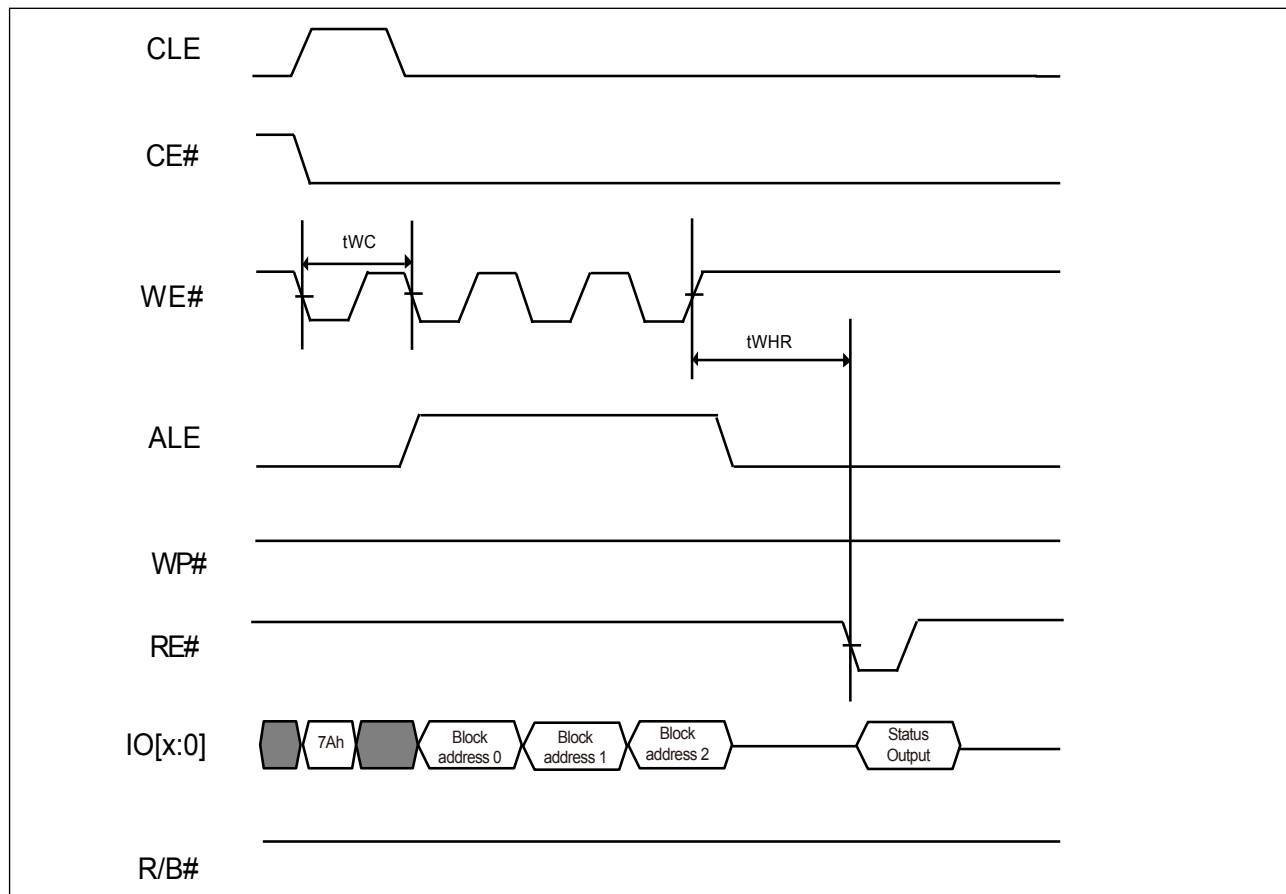
Figure 41. AC Waveforms for Block Protection Status Read
