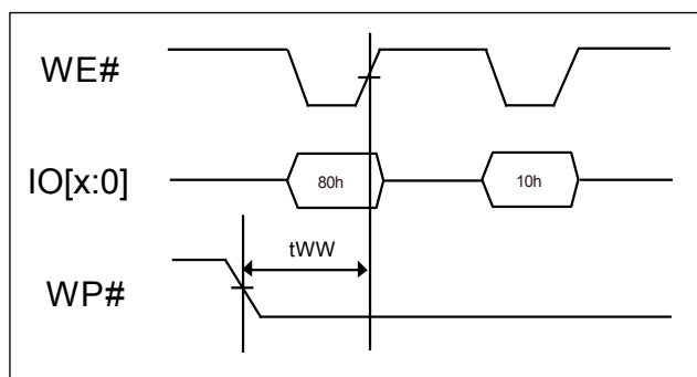
Figure 46-2. Disable Programming of WP# Signal
