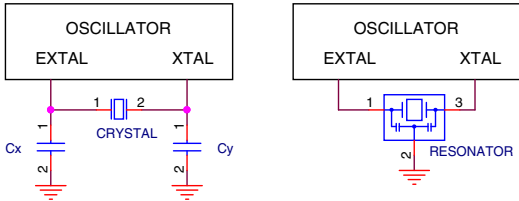
Figure 49. Crystal connection – Diagram 3
