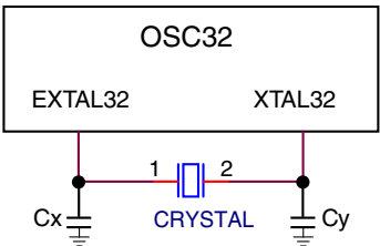
Figure 40. RTC Oscillator (OSC32) module connection – Diagram 1
