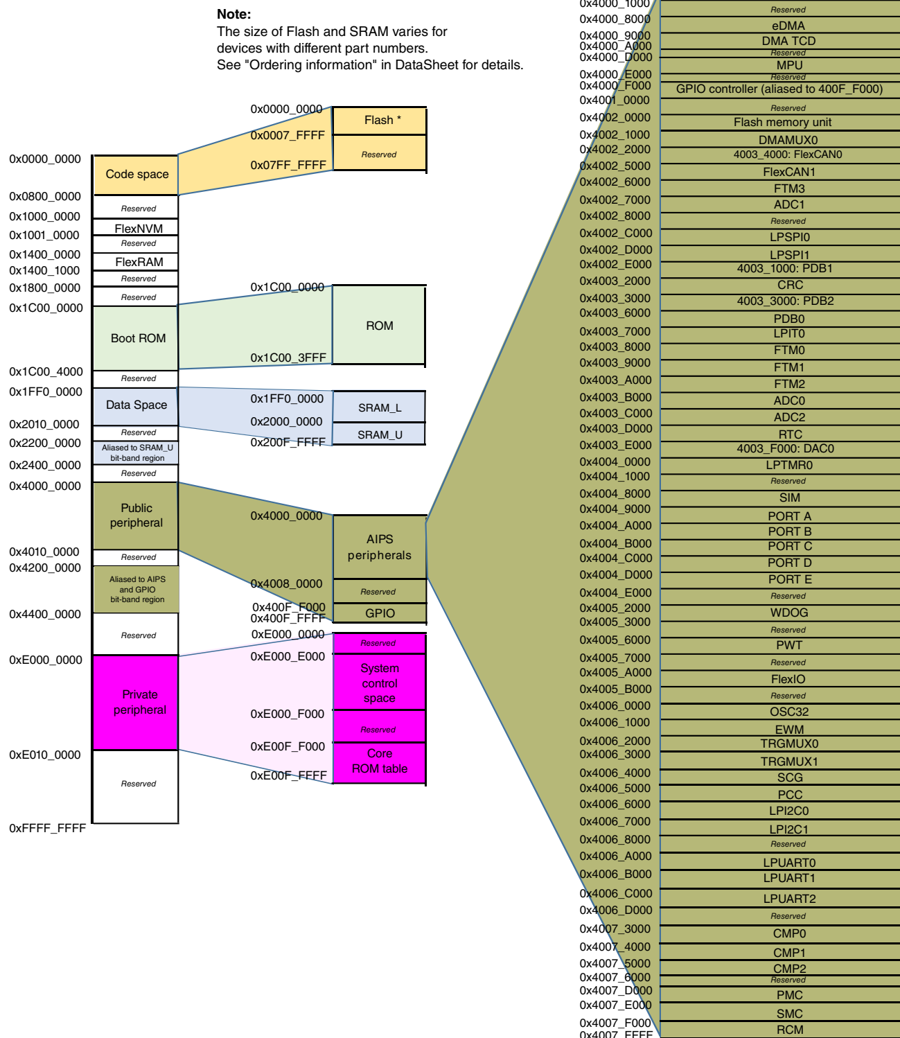
Figure 6. Memory map
