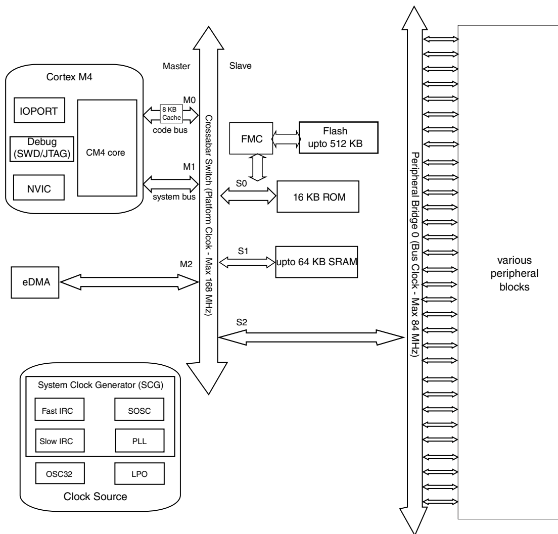
Figure 2. System diagram
