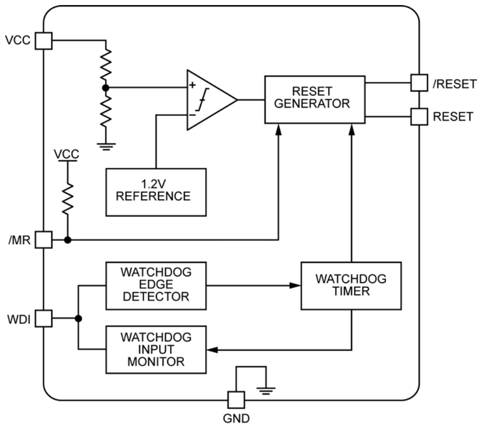
Figure 1. Functional Diagram
