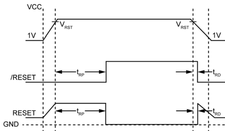
Figure 2. Timing Diagram
