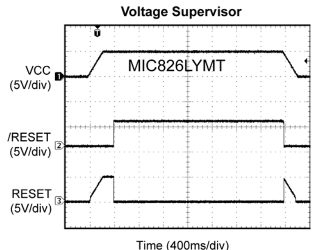
Figure 4. Voltage Supervisor Function
