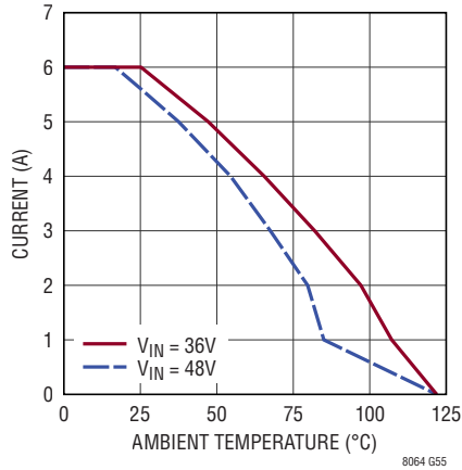
Derating Curve V_{OUT} = 24\text{V}
