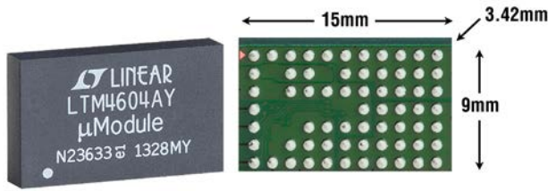
4604A BGA Package
