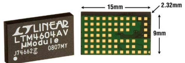
4604A LGA Package
