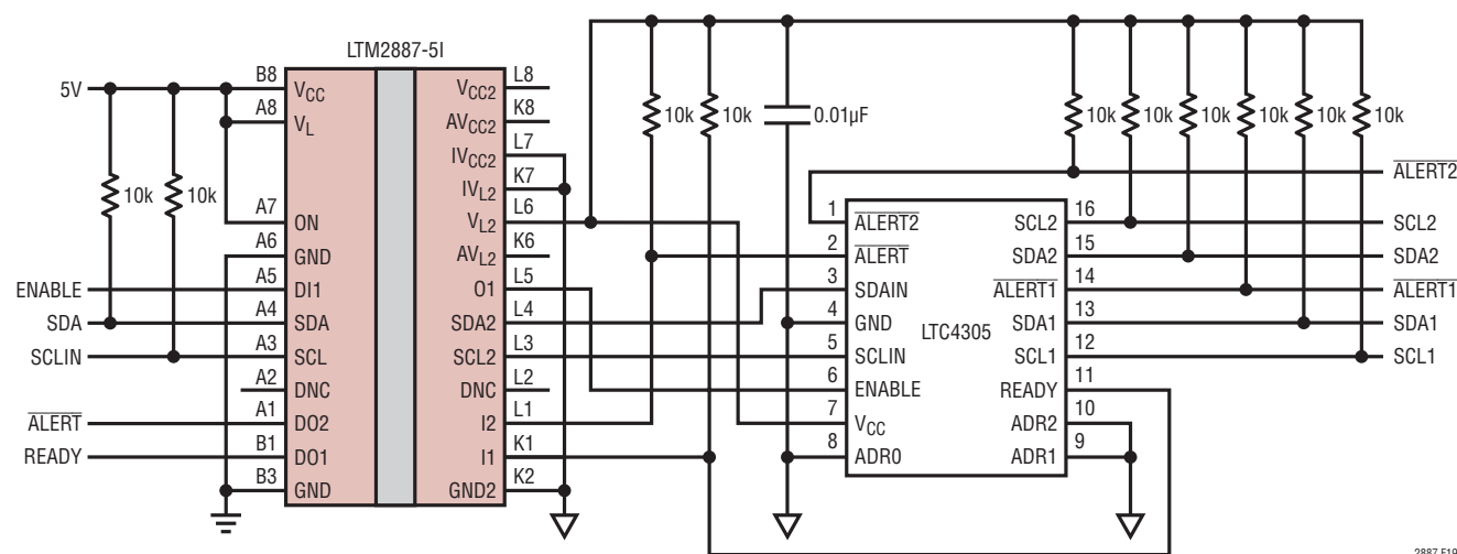
Figure 19. Isolated I²C Buffer with Dual Outputs
