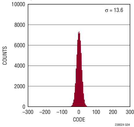
DC Histogram, N = 16, f_{SAMPL} = 2\text{Mps}
