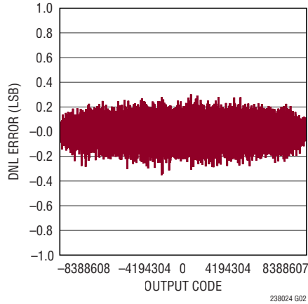
Differential Nonlinearity vs Output Code
