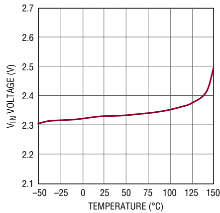
Internal UVLO
