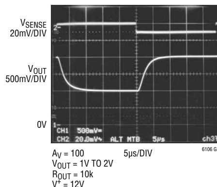
Step Response 10mV to 20mV (RIN = 100Ω)
