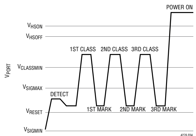
Figure 4. LTPoE++ Detect/Class Signaling Waveform
