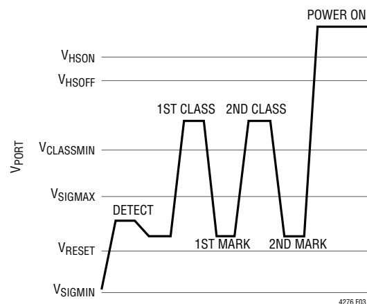
Figure 3. Type 2 Detect/Class Signaling Waveform
