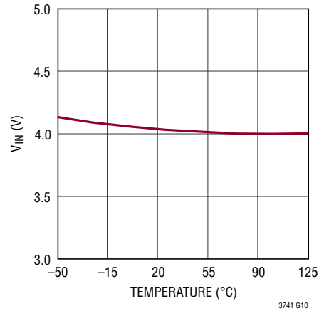
Internal UVLO
