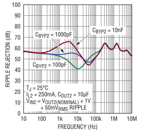
OUT2 Input Ripple Rejection
