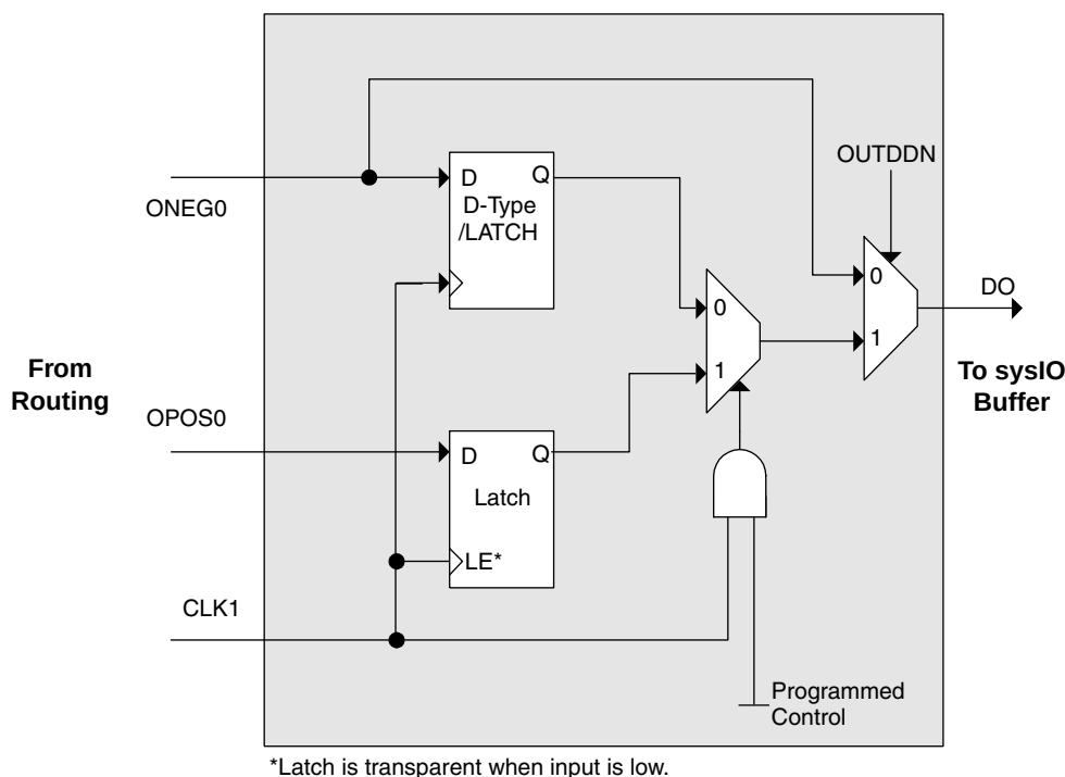
Figure 2-30. ODDRXB Primitive
