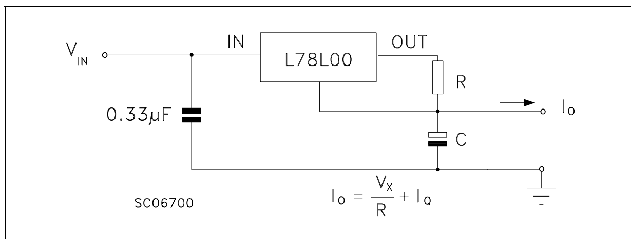
Figure 15: Current Regulator
