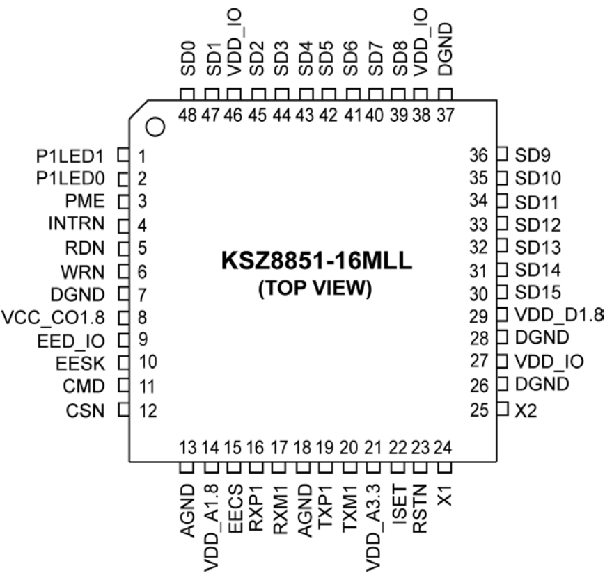
Figure 2. 48-Pin LQFP
