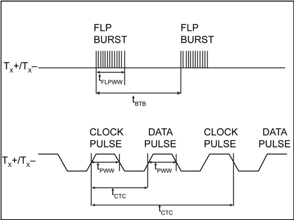
Figure 11. Auto-Negotiation Timing
