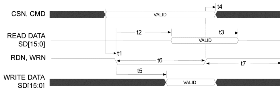
Figure 10. Asynchronous Cycle
