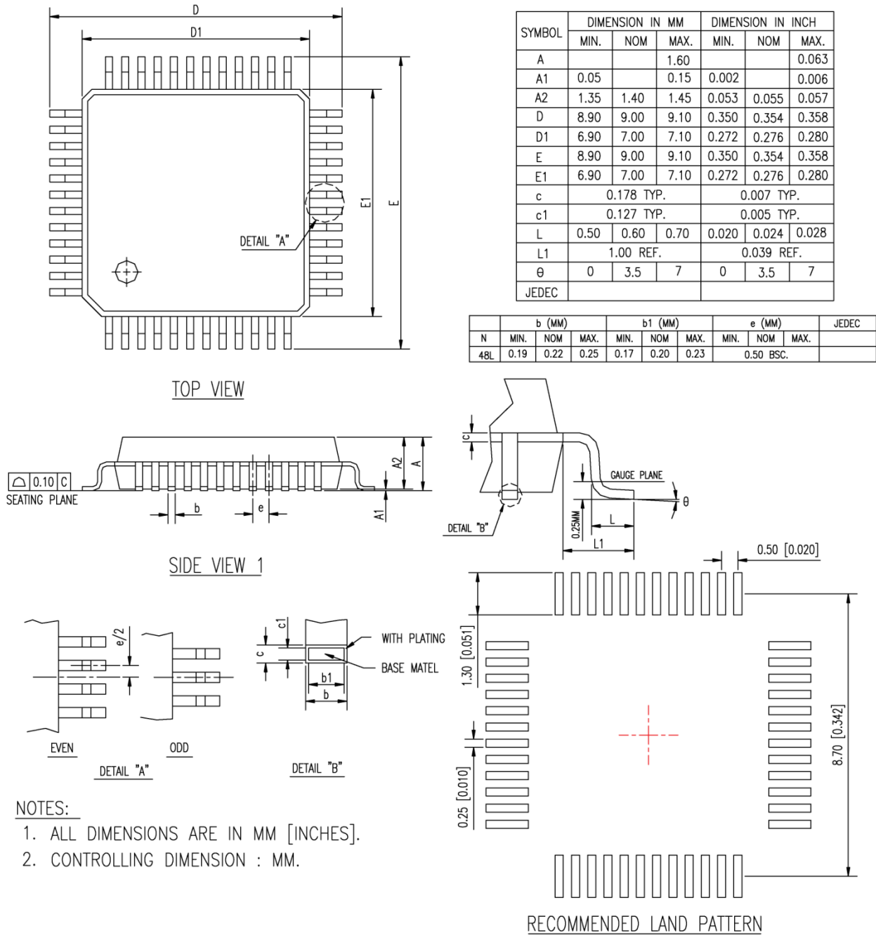
48-Pin (7mm x 7mm) LQFP
