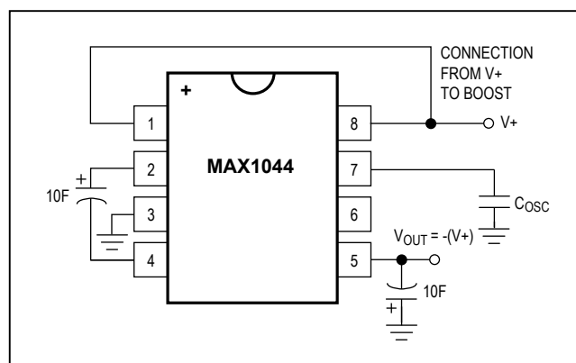
Figure 6. Negative Voltage Converter with C OSC and BOOST
