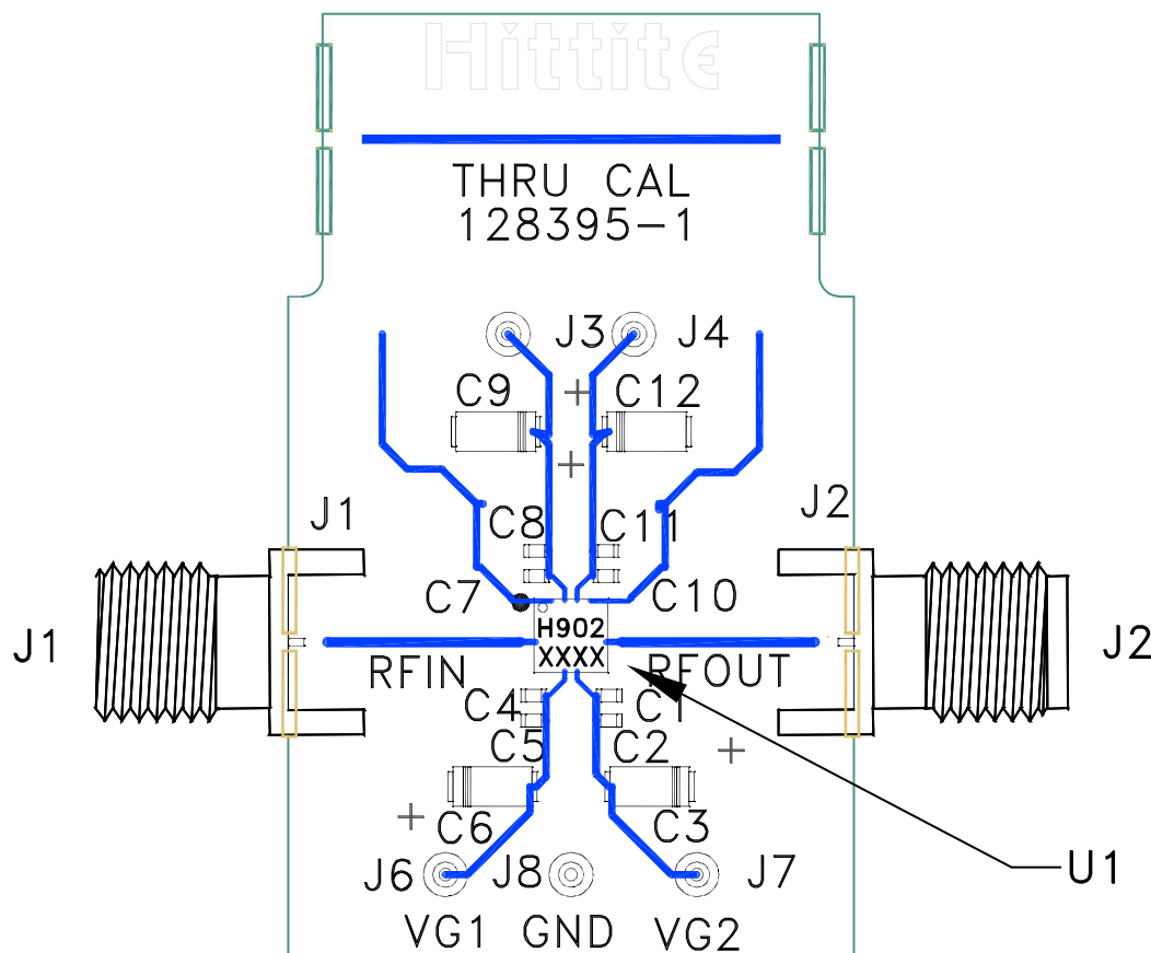
Figure 22. Evaluation PCB (128395-1)
