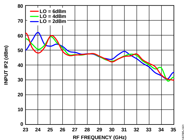
Figure 61. Input IP2 vs. RF Frequency at Various LO Power Levels, T_A = 25^\circ\text{C}
