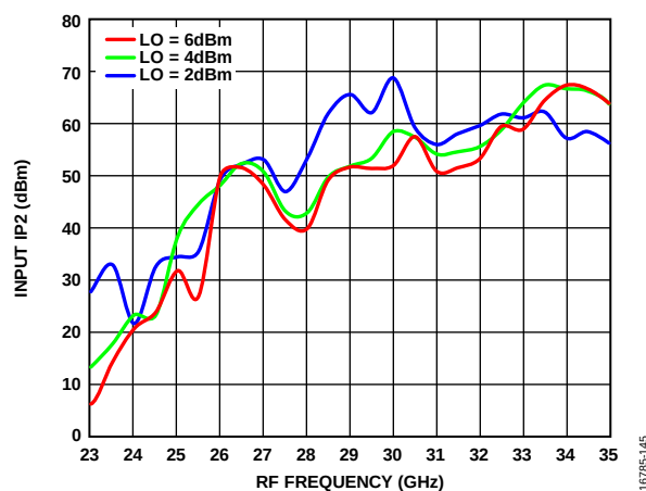
Figure 45. Input IP2 vs. RF Frequency at Various LO Power Levels, TA = 25°C
