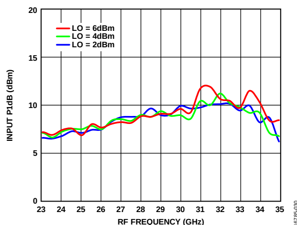
Figure 30. Input P1dB vs. RF Frequency at Various LO Power Levels, T_A = 25^\circ\text{C}
