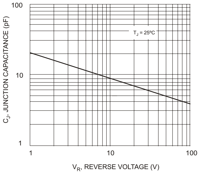
V_R , REVERSE VOLTAGE (V) Fig. 3, Capacitance Characteristics
