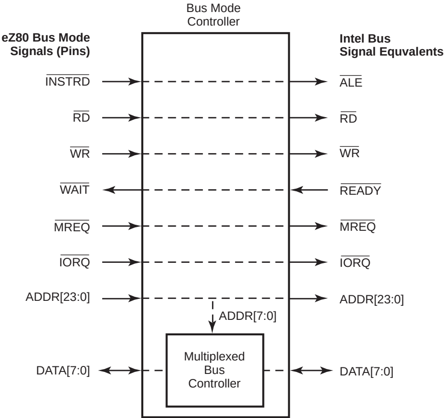
Figure 9. Intel® Bus Mode Signal and Pin Mapping
