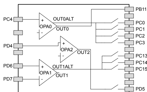
Figure 5.7. Opamp Pinout
