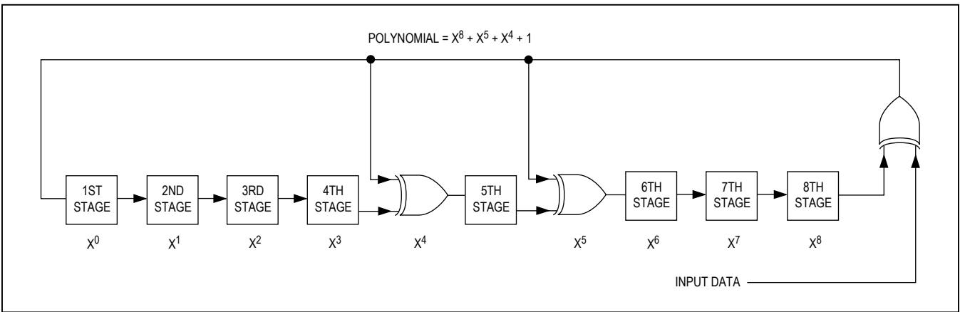
Figure 5. CRC Polynomial
