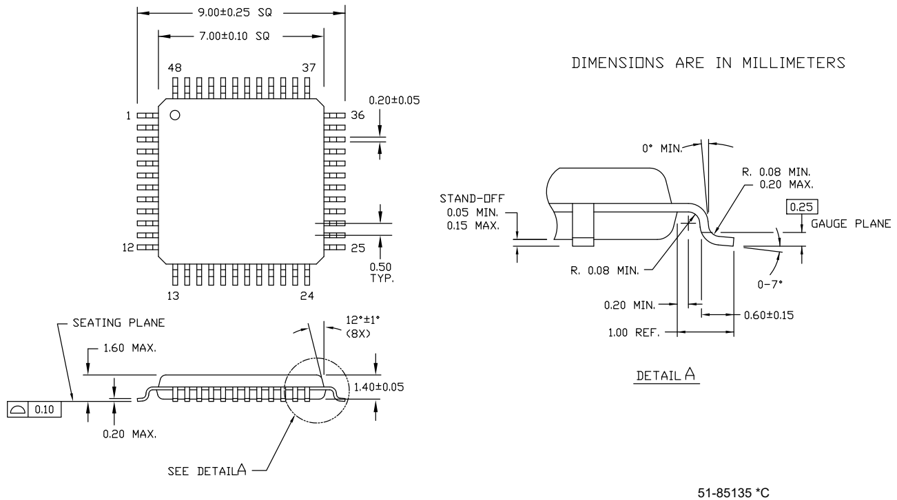
Figure 6. 48-pin TQFP (7 × 7 × 1.4 mm) Package Outline, 51-85135
