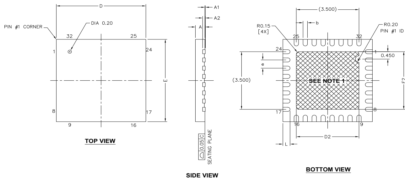
Figure 19. 32-Pin ( 5 \times 5 \times 0.6 mm) QFN
