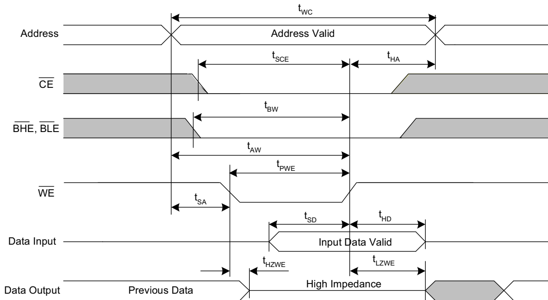
Figure 7. SRAM Write Cycle No. 1 ( \overline{\text{WE}} Controlled) [21, 22, 23]
