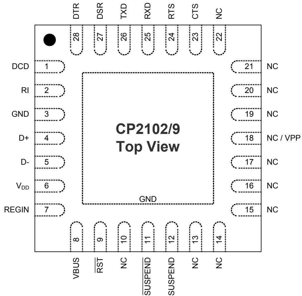
Figure 2. QFN-28 Pinout Diagram (Top View)
