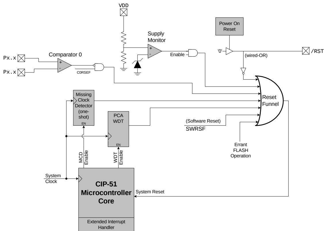
Figure 12.1. Reset Sources
