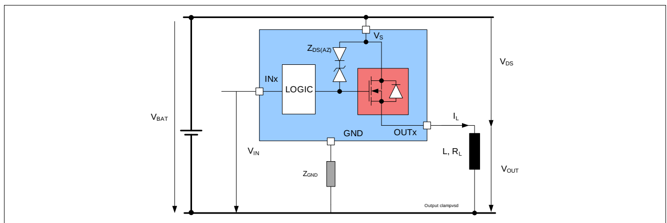
Figure 8 Output Clamp
