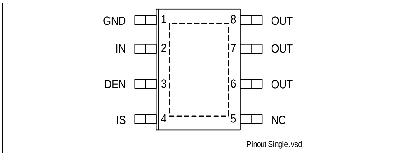
Figure 1 Pin Configuration
