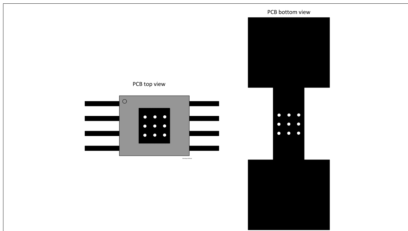
Figure 3 PC Board Top and Bottom View for Thermal Simulation with 600 mm 2 Cooling Area
