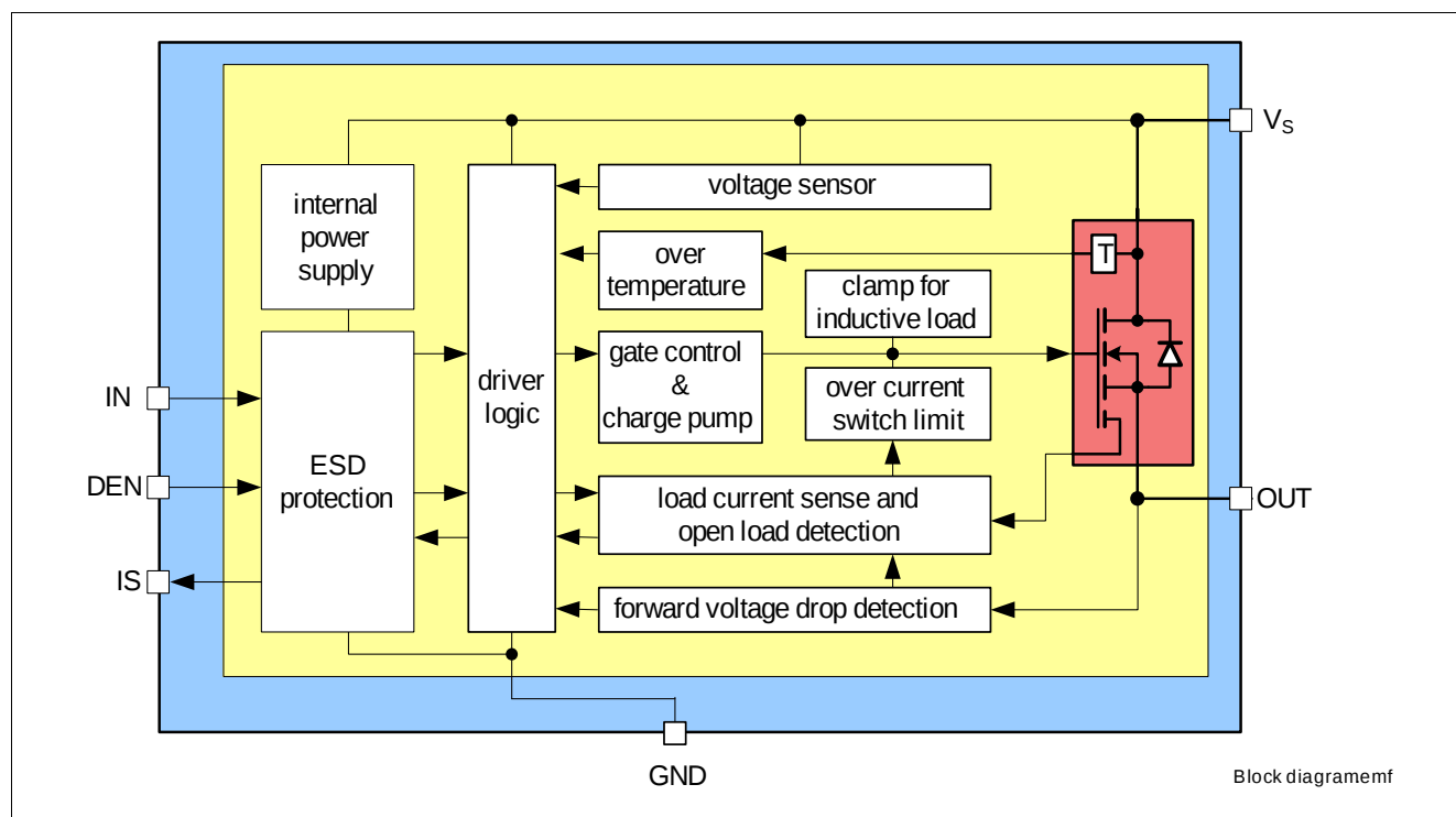
Figure 1 Block Diagram for the BTS5200-1EJA
