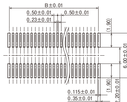
Recommended metal mask pattern Metal mask thickness: When 120 \mu m (Opening area ratio: 87%)
