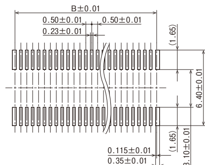
Recommended metal mask pattern Metal mask thickness: When 120 \mu m (Opening area ratio: 76%)
