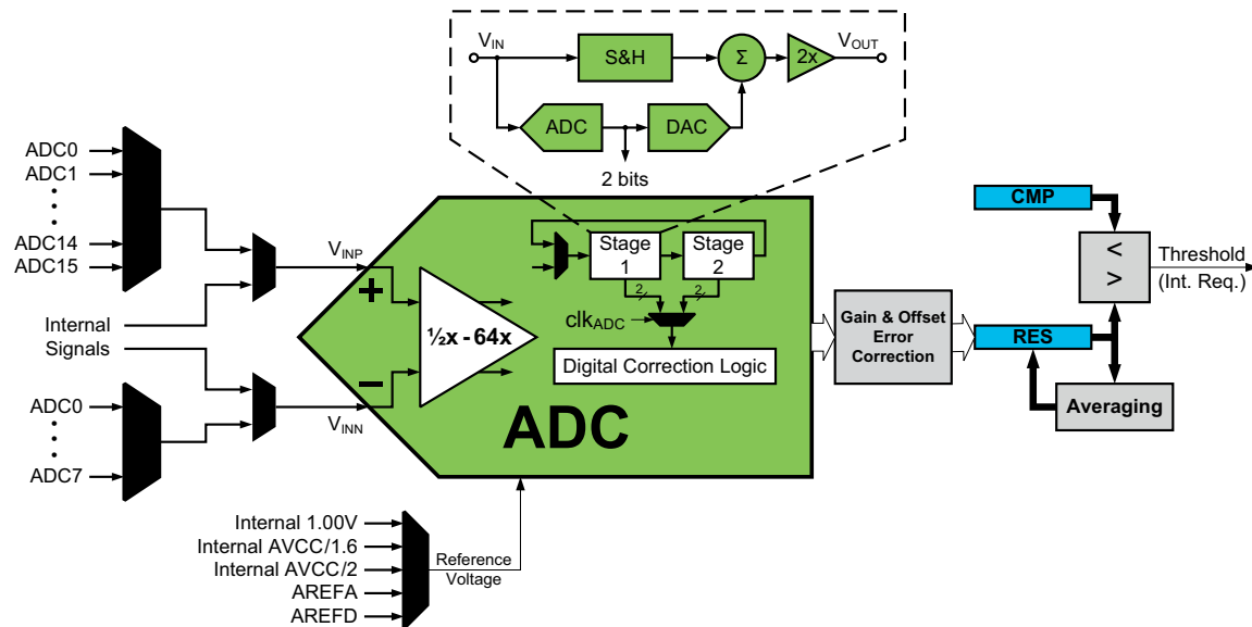
Figure 28-1. ADC Overview
