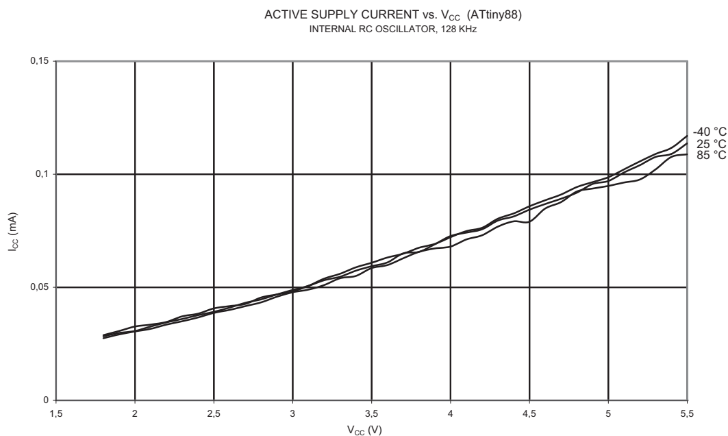
Figure 23-62. Active Supply Current vs. V_{CC} (Internal Oscillator, 128 kHz)
