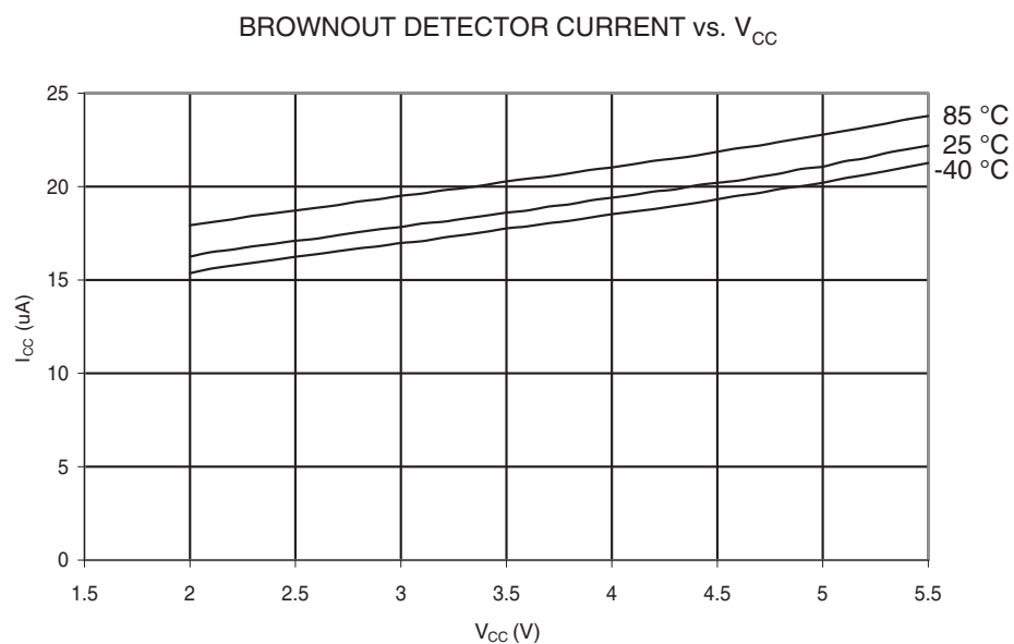
Figure 23-15. Brownout Detector Current vs. V_{CC}
