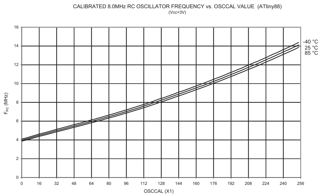
Figure 23-114. Calibrated 8 MHz Oscillator Frequency vs. OSCCAL Value
