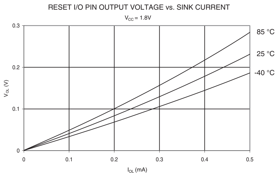
Figure 23-34. V_{OL} : Reset Pin Output Voltage vs. Sink Current ( V_{CC} = 1.8V )
