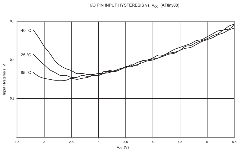
Figure 23-99. V_{IH}-V_{IL} : I/O Pin Input Hysteresis vs. V_{CC}
