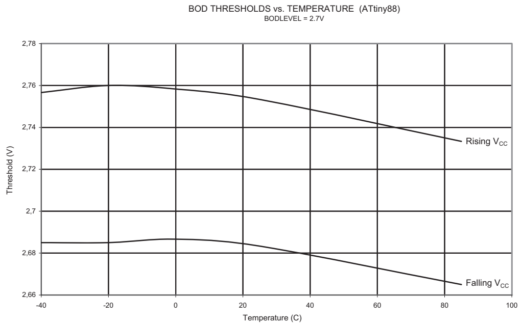
Figure 23-104. BOD Threshold vs. Temperature (BOD Level is 2.7V)
