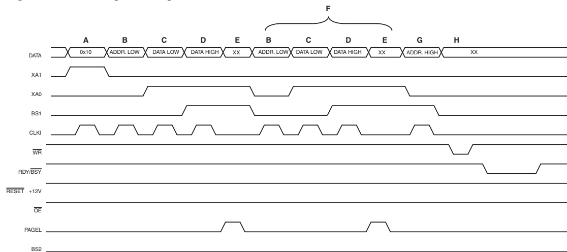
Figure 21-3. Programming the Flash Waveforms
