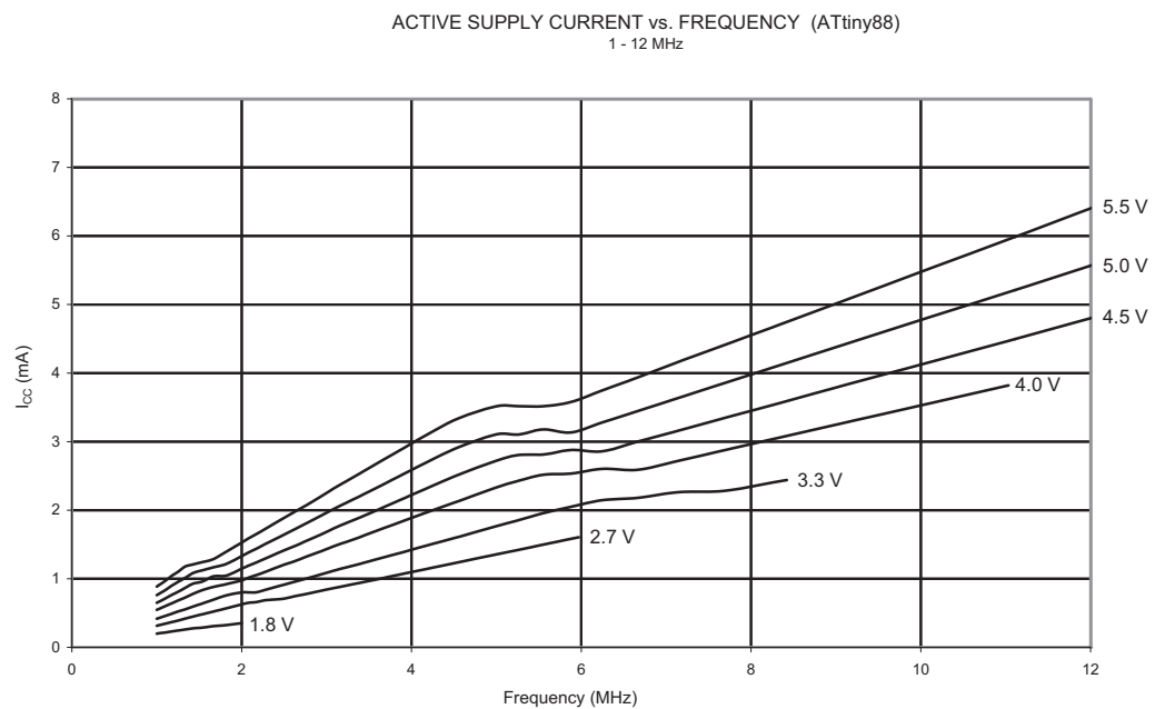
Figure 23-59. Active Supply Current vs. Frequency (1 - 12 MHz)
