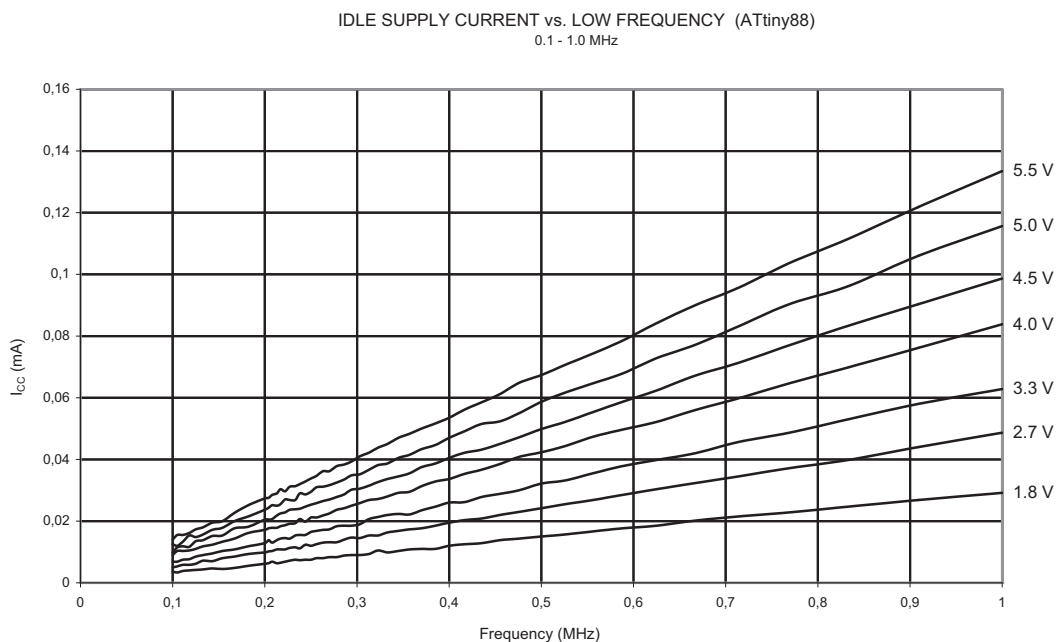
Figure 23-63. Idle Supply Current vs. low Frequency (0.1 - 1.0 MHz)
