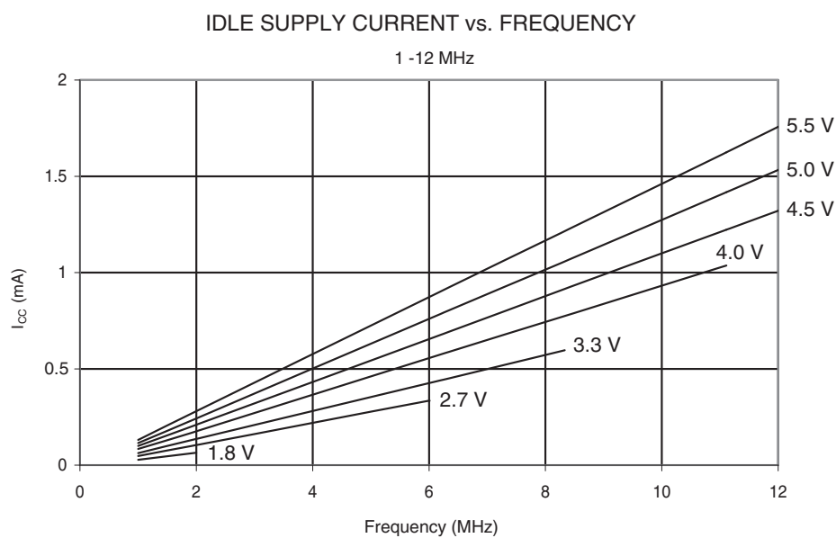
Figure 23-7. Idle Supply Current vs. Frequency (1 - 12 MHz)
