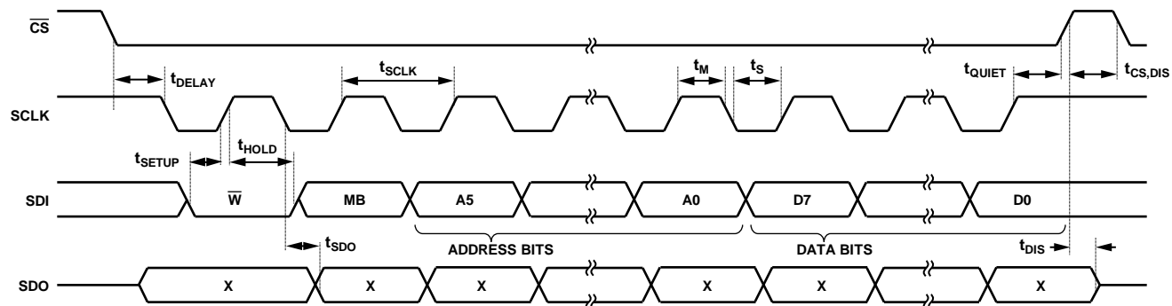
Figure 52. SPI 4-Wire Write
