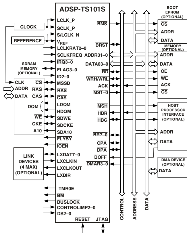
Figure 2. Single-Processor System with External SDRAM
