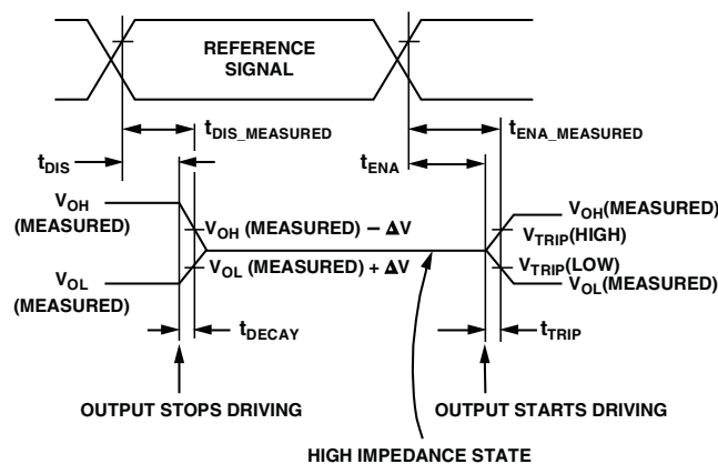
Figure 66. Output Enable/Disable
