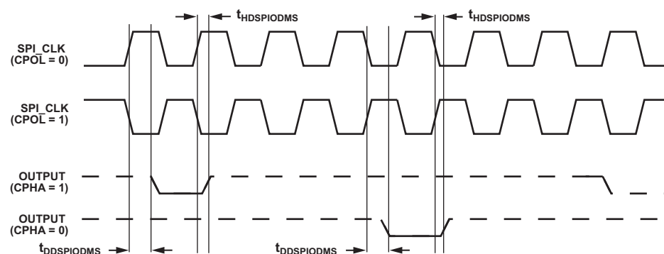
Figure 45. ODM Slave
