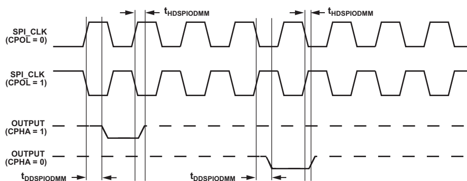
Figure 44. ODM Master
