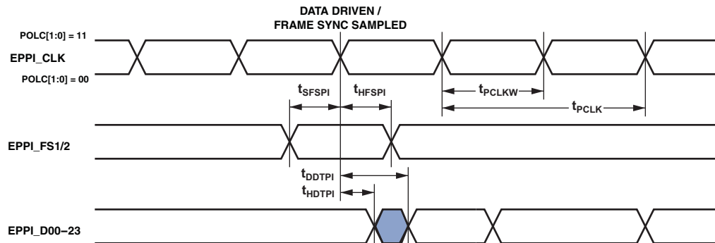
Figure 28. PPI Internal Clock GP Transmit Mode with External Frame Sync Timing
