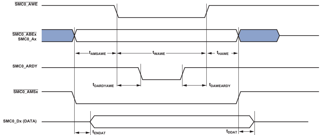
Figure 16. Asynchronous Write
