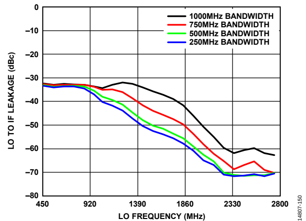
Figure 50. LO to IF Rejection for LO Frequency at 100 MHz and a Low-Pass Filter Setting of 250 MHz
