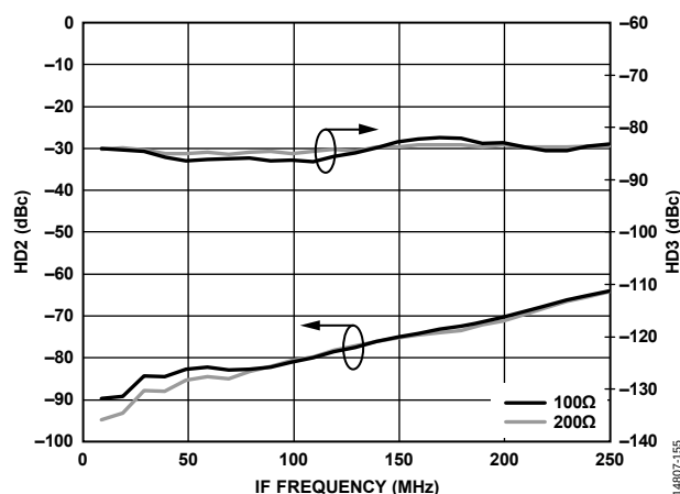
Figure 55. HD2 and HD3 vs. IF Frequency for Different Loads
