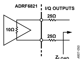
Figure 51. IF Output Schematic
