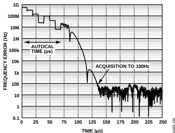
Figure 58. PLL Acquisition
