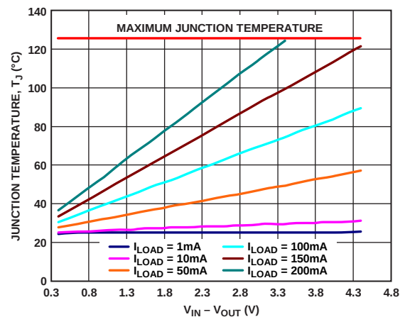
Figure 48. 100 mm² of PCB Copper, TSOT, T_A = 25^\circ\text{C}
