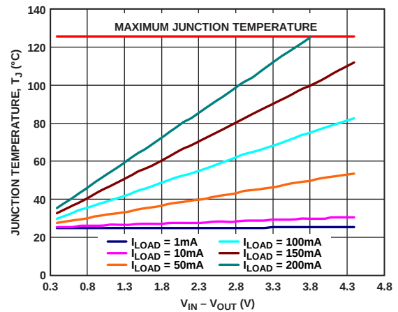
Figure 47. 500 mm² of PCB Copper, TSOT, T_A = 25^\circ\text{C}
