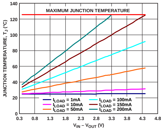
Figure 43. 500 mm² of PCB Copper, WLCSP, T_A = 25^\circ\text{C}
