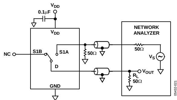
Figure 22. Off Isolation
