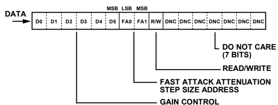
Figure 49. 16-Bit SPI Register
