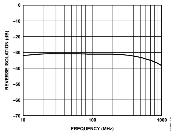
Figure 41. Reverse Isolation vs. Frequency
