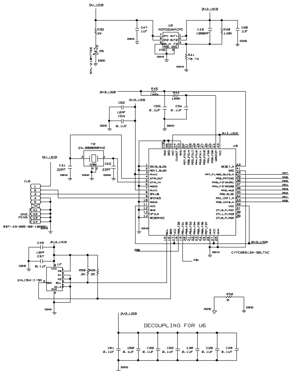
Figure 61. Logic Schematic
