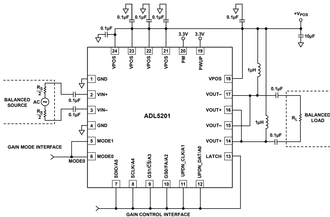
Figure 53. Basic Connections
