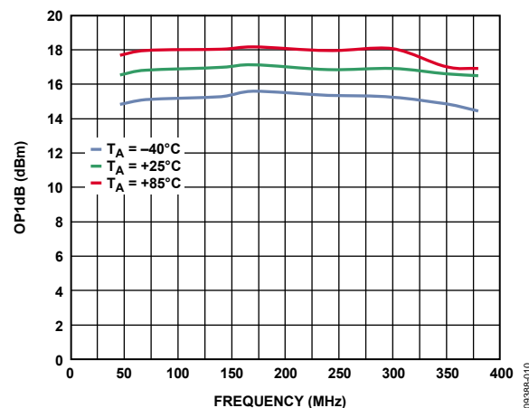
Figure 11. OP1dB vs. Frequency at Maximum Gain, Three Temperatures
