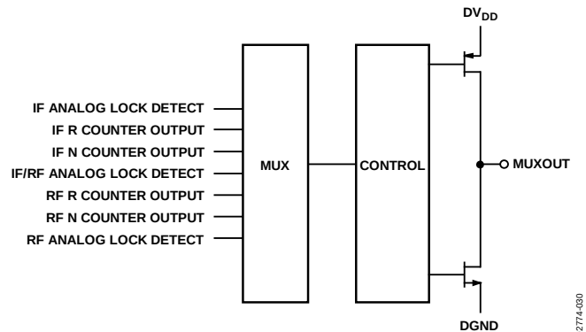
Figure 30. MUXOUT Schematic
