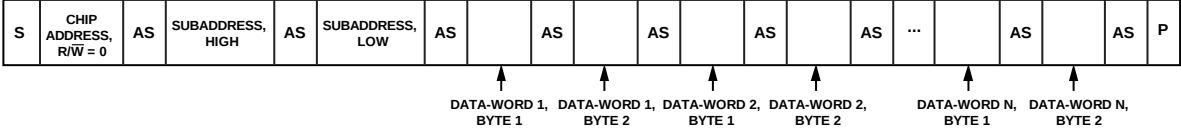
Figure 16. Burst Mode I²C Write Sequence
