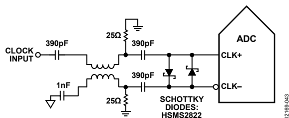
Figure 61. Balun-Coupled Differential Clock (Up to 1240 MHz)
