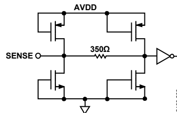
Figure 50. Equivalent SENSE Circuit
