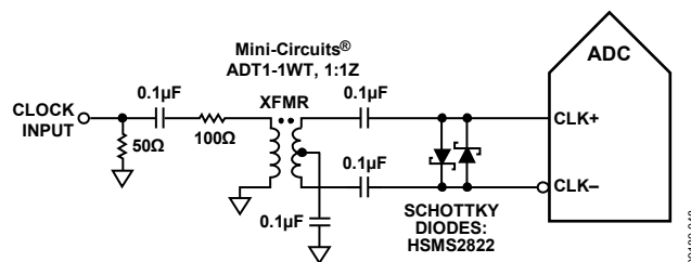
Figure 54. Transformer-Coupled Differential Clock (Up to 200 MHz)
